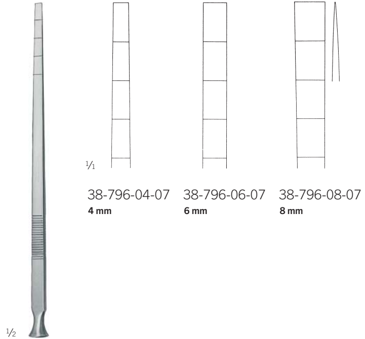
Epker 38-796-04-07 - 38-796-08-07 18 cm / 7 1 / 8 "
